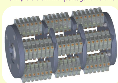
Komplett dob 5 sarkú lamellákkal Complete drum with pentagonal cutters
